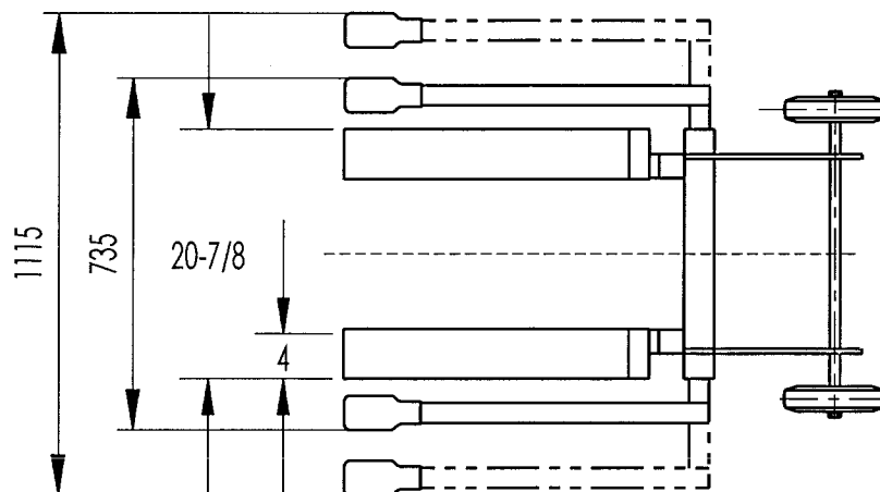
A-LIFT-S/A-LIFT-S-HP
