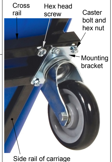
FIG. 1B: Attach casters
