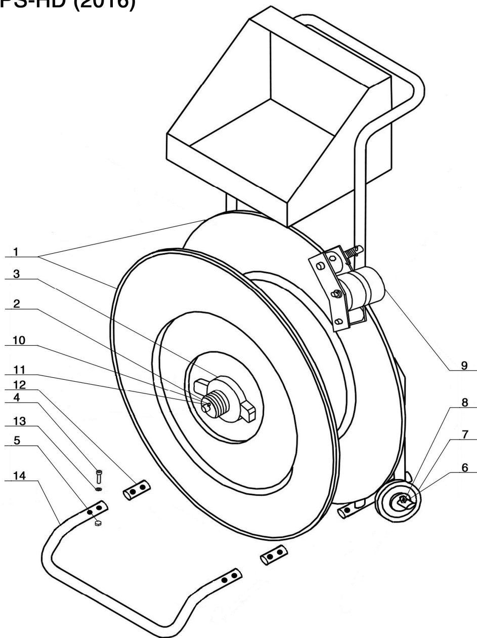
Main Assembly Parts List
