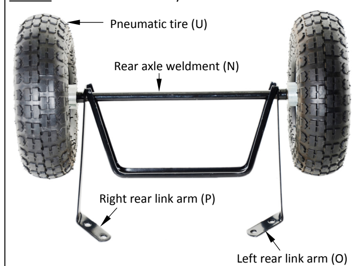
FIG. 2A: Rear wheel assembly
