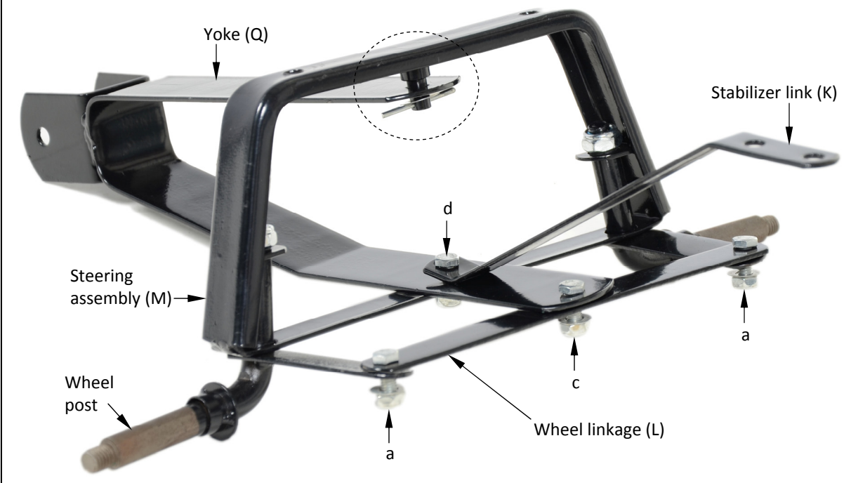
FIG. 1: Steering mechanism
