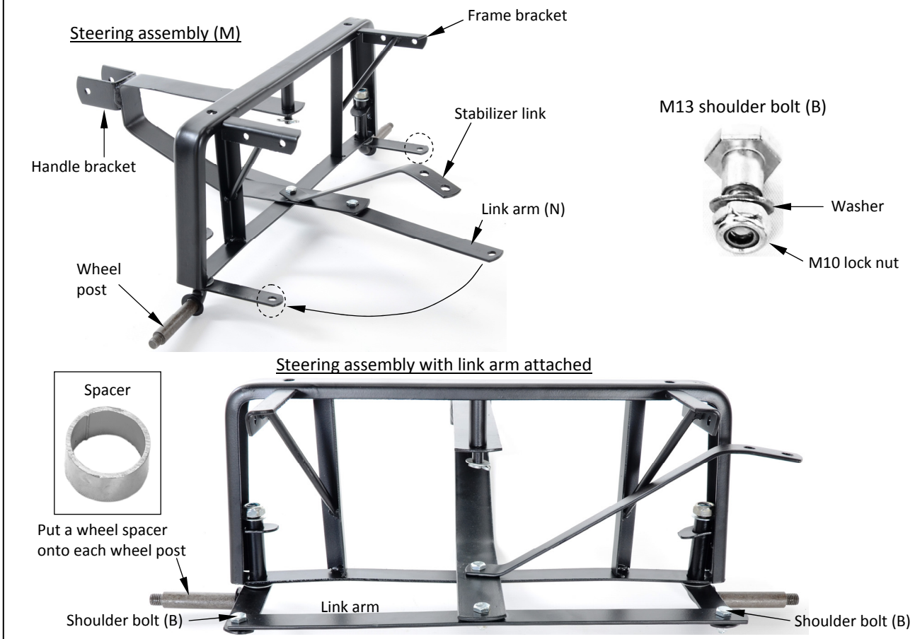
FIG. 1: Complete the steering assembly
