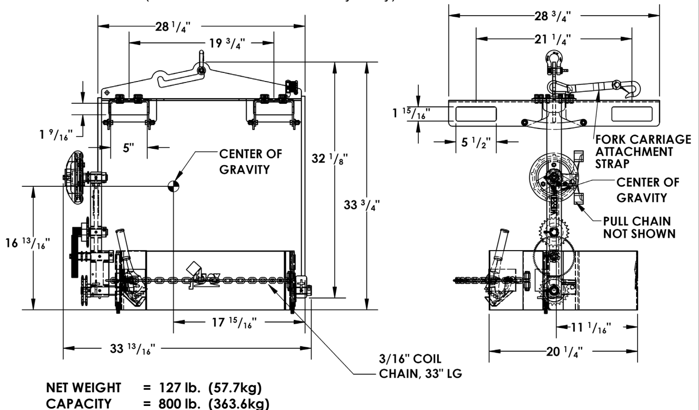
DCT-85-4WFP (Bolt-on Fork Pockets for 4-way Entry)
