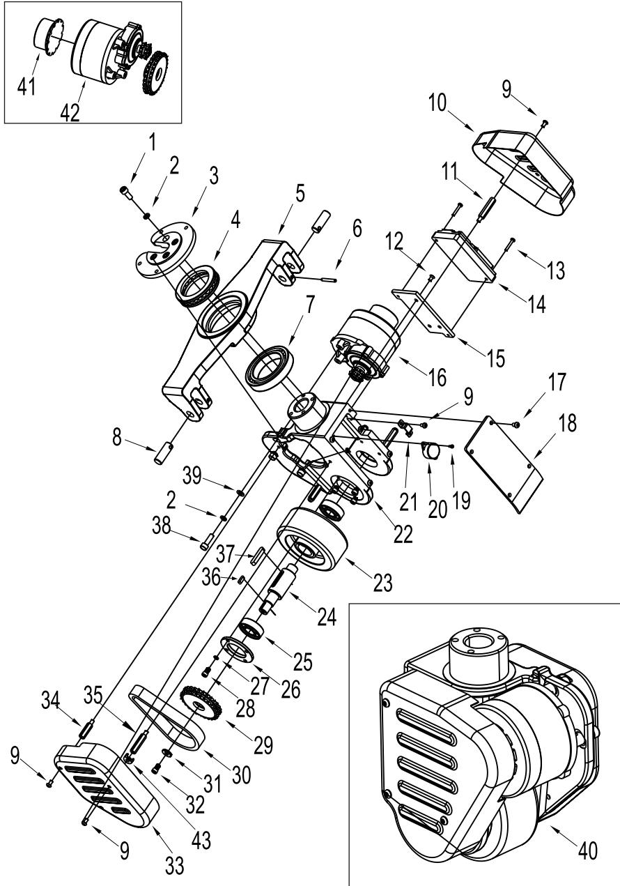
Fig. 2 Driving system
