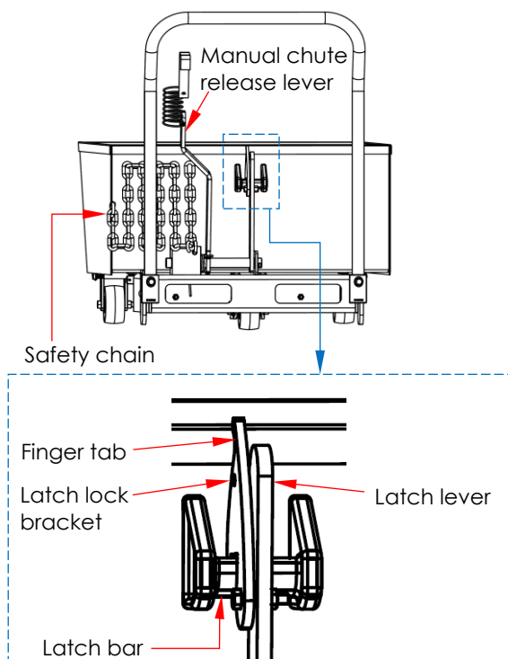
Diagram 1: Unlock the latch
